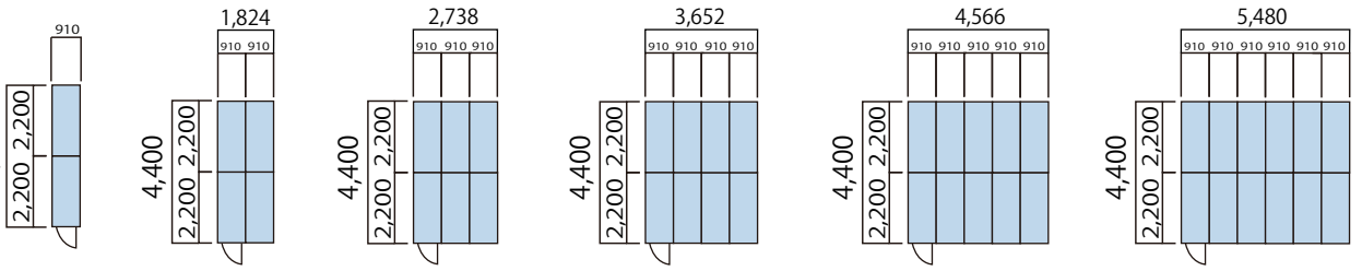
KJ-2連棟 KJ-4連棟 KJ-6連棟 KJ-8連棟 KJ-10連棟 KJ-12連棟
